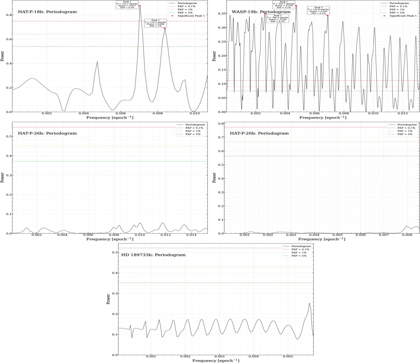
Figure 16. from Yunke Wu et al 2026 Astrophys. J. Suppl. 287 doi:10.3847/1538-4365/aea075 https://dx.doi.org/10.3847/1538-4365/aea075 © 2026. The Author(s). Published by the American Astronomical Society.
