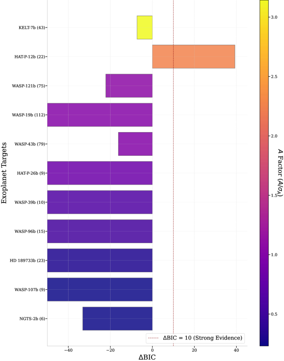
Figure 12. from Yunke Wu et al 2026 Astrophys. J. Suppl. 287 doi:10.3847/1538-4365/aea075 https://dx.doi.org/10.3847/1538-4365/aea075 © 2026. The Author(s). Published by the American Astronomical Society.
