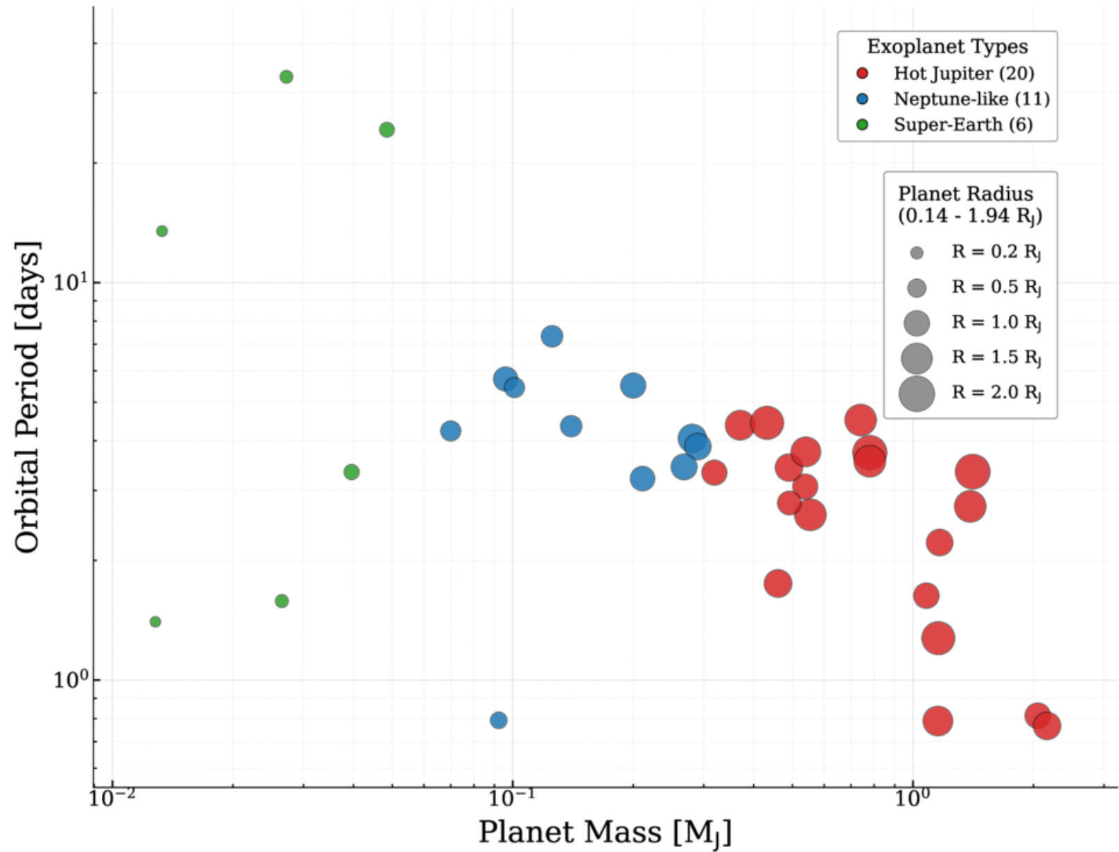
Figure 1. from Yunke Wu et al 2026 Astrophys. J. Suppl. 287 doi:10.3847/1538-4365/aea075 https://dx.doi.org/10.3847/1538-4365/aea075 © 2026. The Author(s). Published by the American Astronomical Society.
