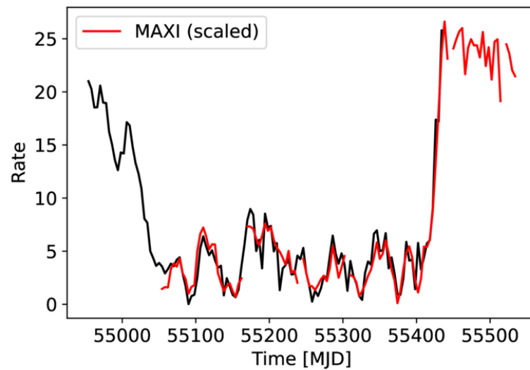
Figure C1. from Eric Miao et al 2026 Astrophys. J. Suppl. 286 doi:10.3847/1538-4365/ae9f56 https://dx.doi.org/10.3847/1538-4365/ae9f56 © 2026. The Author(s). Published by the American Astronomical Society.
