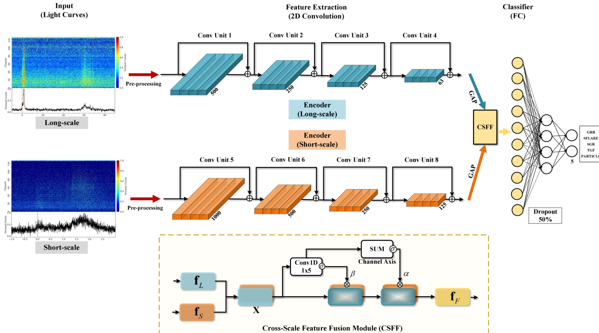
Figure 2. from Peng Zhang et al 2026 Astrophys. J. Suppl. 286 doi:10.3847/1538-4365/ae9cb1 https://dx.doi.org/10.3847/1538-4365/ae9cb1 © 2026. The Author(s). Published by the American Astronomical Society.
