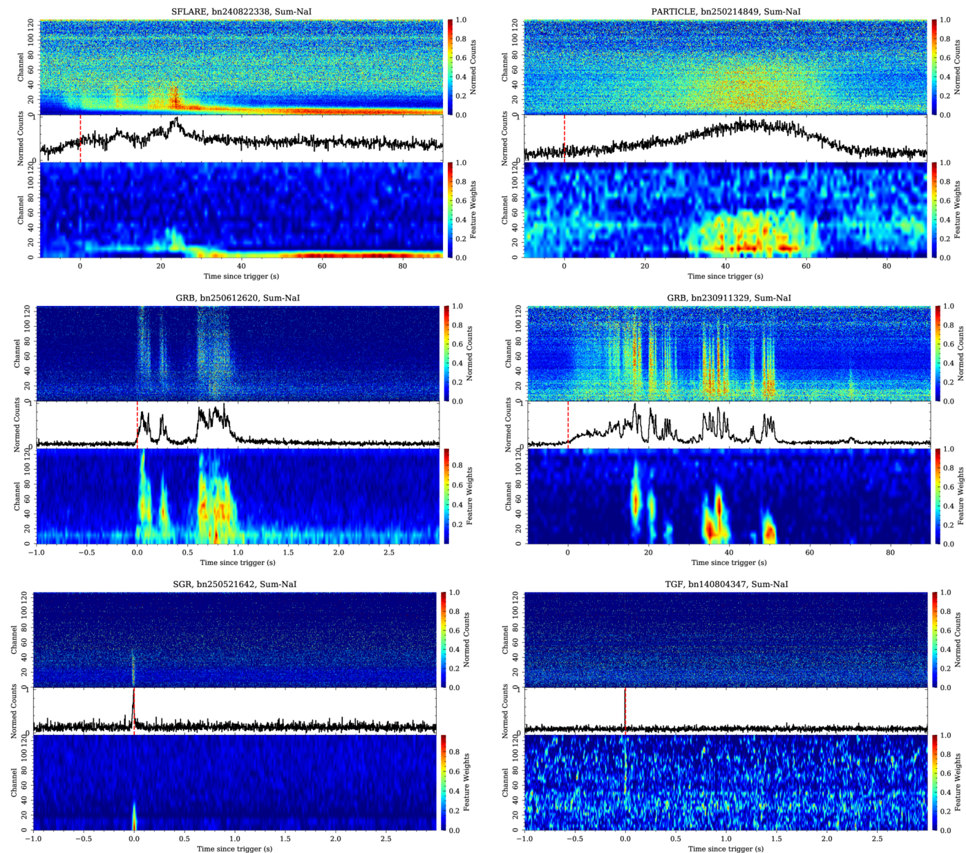
Figure 1. from Peng Zhang et al 2026 Astrophys. J. Suppl. 286 doi:10.3847/1538-4365/ae9cb1 https://dx.doi.org/10.3847/1538-4365/ae9cb1 © 2026. The Author(s). Published by the American Astronomical Society.
