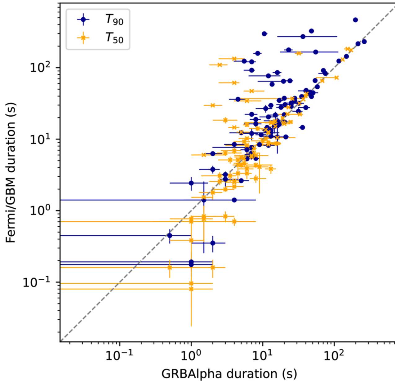
Figure 9. from Marianna Dafiřková et al 2026 Astrophys. J. Suppl. 286 doi:10.3847/1538-4365/ae9c3b https://dx.doi.org/10.3847/1538-4365/ae9c3b © 2026. The Author(s). Published by the American Astronomical Society.
