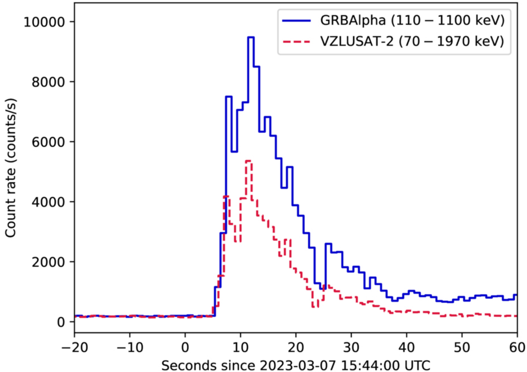
Figure 8. from Marianna Daříková et al 2026 Astrophys. J. Suppl. 286 doi:10.3847/1538-4365/ae9c3b https://dx.doi.org/10.3847/1538-4365/ae9c3b © 2026. The Author(s). Published by the American Astronomical Society.
