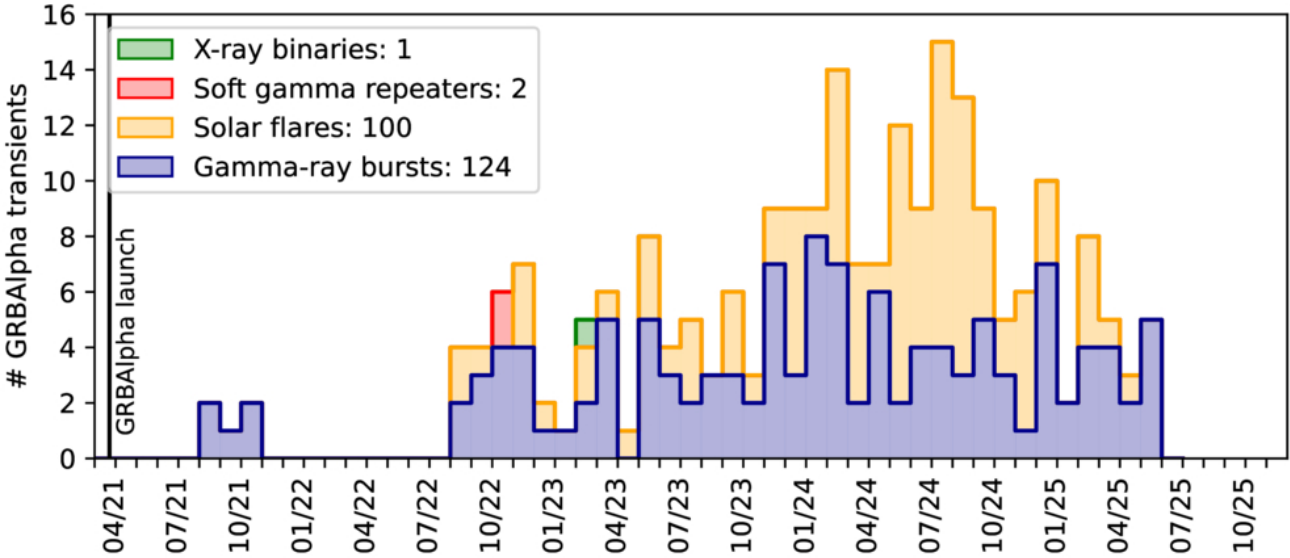
Figure 4. from Marianna Daříková et al 2026 Astrophys. J. Suppl. 286 doi:10.3847/1538-4365/ae9c3b https://dx.doi.org/10.3847/1538-4365/ae9c3b © 2026. The Author(s). Published by the American Astronomical Society.
