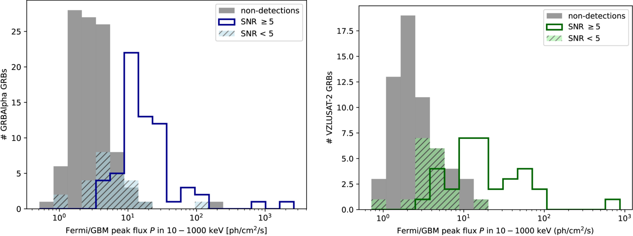
Figure 13. from Marianna Daříková et al 2026 Astrophys. J. Suppl. 286 doi:10.3847/1538-4365/ae9c3b https://dx.doi.org/10.3847/1538-4365/ae9c3b © 2026. The Author(s). Published by the American Astronomical Society.
