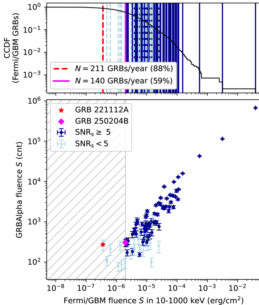
Figure 12. from Marianna Dafíková et al 2026 Astrophys. J. Suppl. 286 doi:10.3847/1538-4365/ae9c3b https://dx.doi.org/10.3847/1538-4365/ae9c3b © 2026. The Author(s). Published by the American Astronomical Society.
