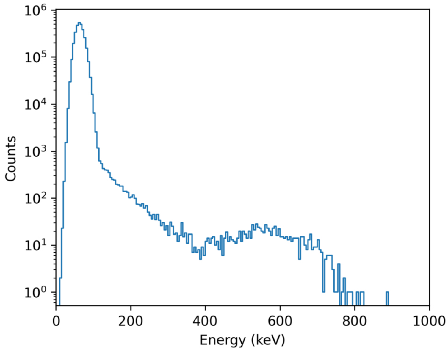
Figure 1. from Marianna Daříková et al 2026 Astrophys. J. Suppl. 286 doi:10.3847/1538-4365/ae9c3b https://dx.doi.org/10.3847/1538-4365/ae9c3b © 2026. The Author(s). Published by the American Astronomical Society.
