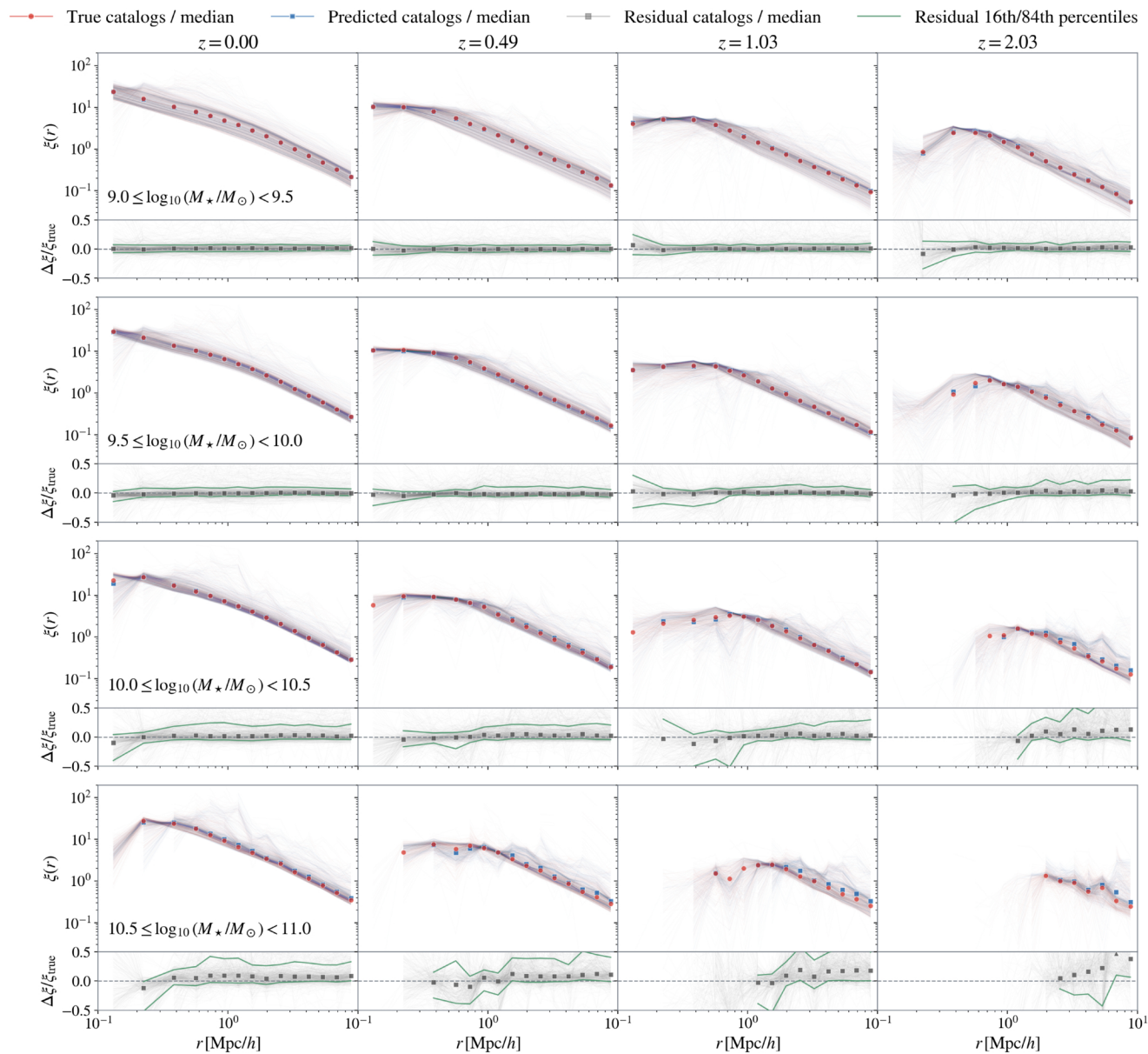
Figure 6. from Xuejie Li et al 2026 Astrophys. J. Suppl. 286 doi:10.3847/1538-4365/ae9a75 https://dx.doi.org/10.3847/1538-4365/ae9a75 © 2026. The Author(s). Published by the American Astronomical Society.
