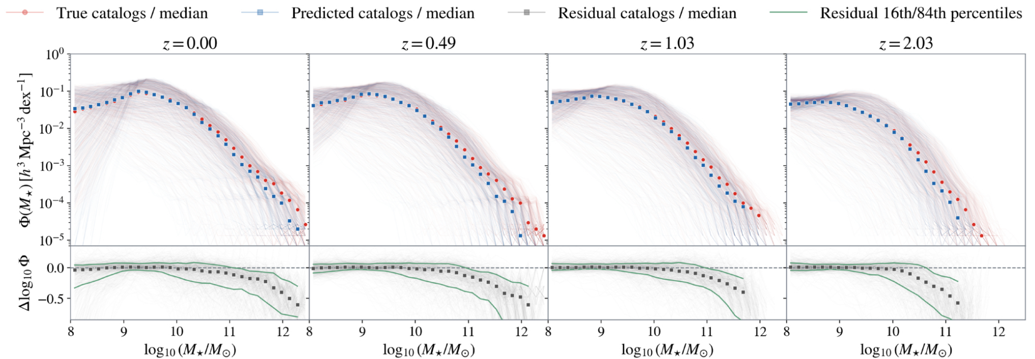
Figure 5. from Xuejie Li et al 2026 Astrophys. J. Suppl. 286 doi:10.3847/1538-4365/ae9a75 https://dx.doi.org/10.3847/1538-4365/ae9a75 © 2026. The Author(s). Published by the American Astronomical Society.
