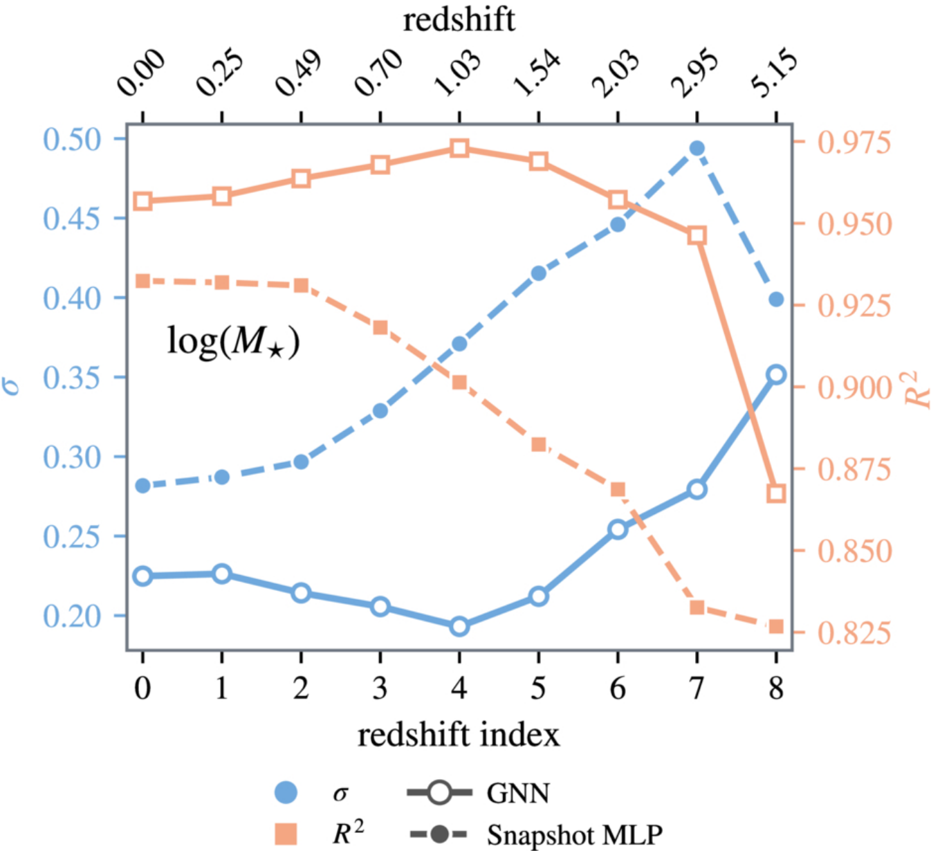
Figure 4. from Xuejie Li et al 2026 Astrophys. J. Suppl. 286 doi:10.3847/1538-4365/ae9a75 https://dx.doi.org/10.3847/1538-4365/ae9a75 © 2026. The Author(s). Published by the American Astronomical Society.
