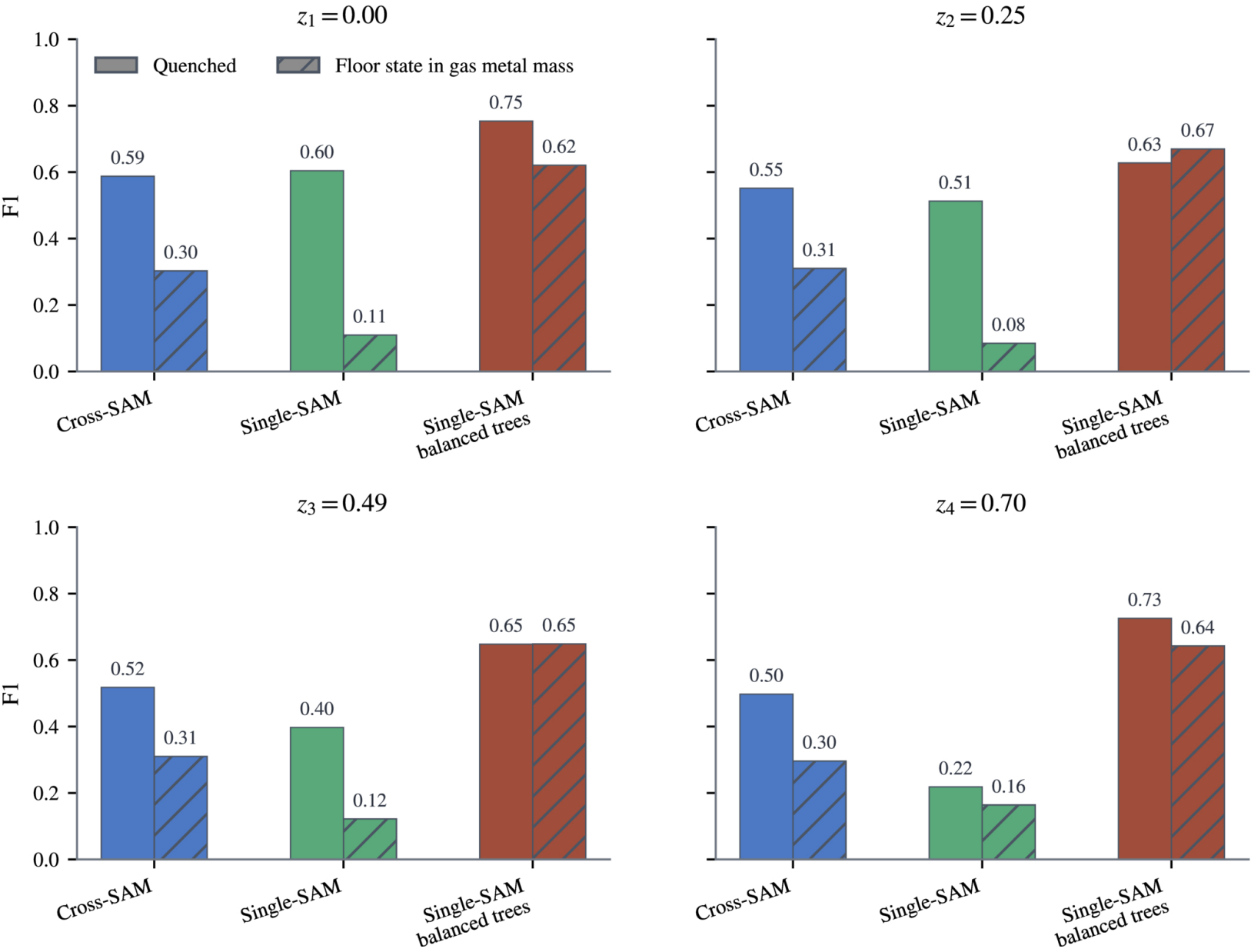
Figure 13. from Xuejie Li et al 2026 Astrophys. J. Suppl. 286 doi:10.3847/1538-4365/ae9a75 https://dx.doi.org/10.3847/1538-4365/ae9a75 © 2026. The Author(s). Published by the American Astronomical Society.
