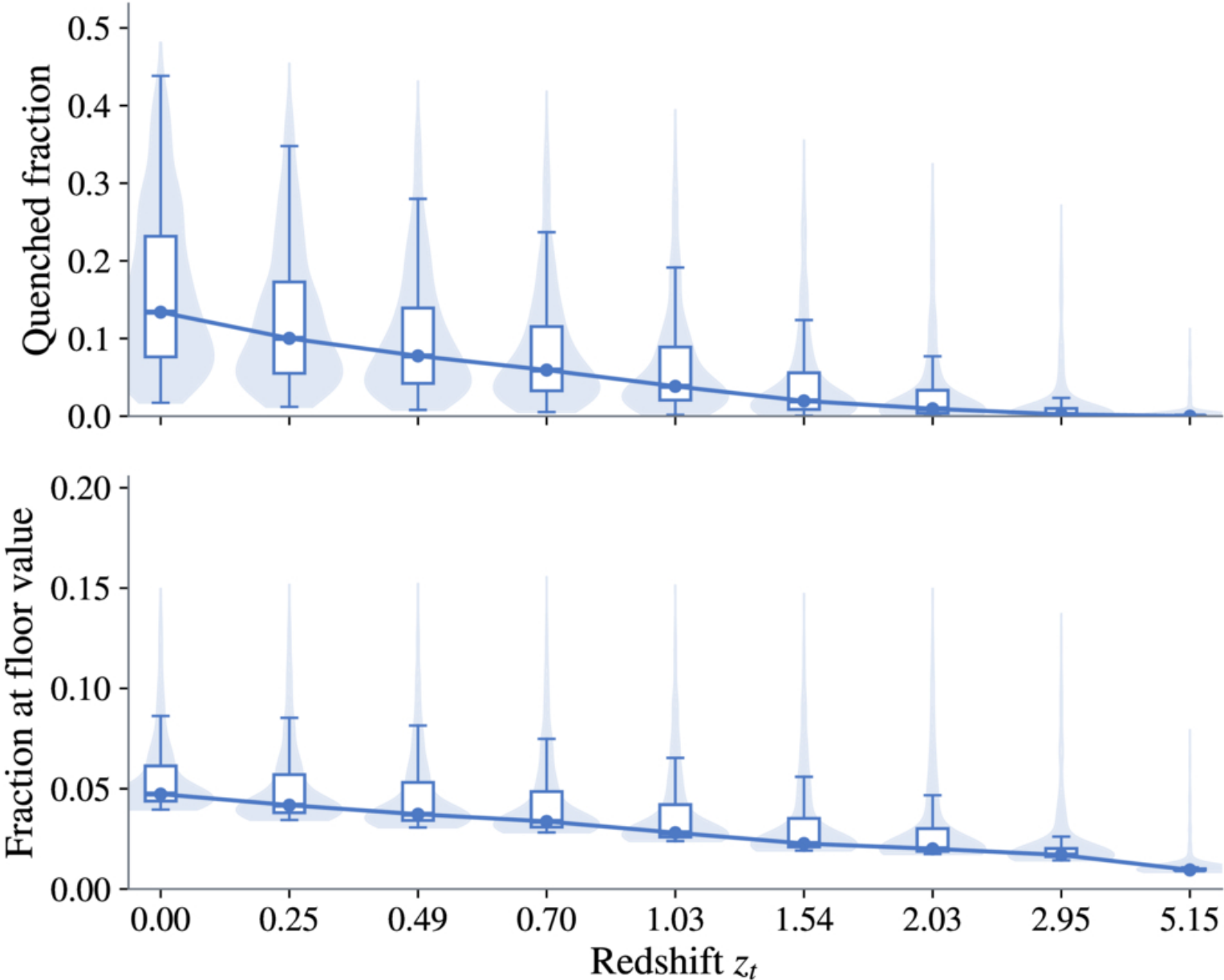
Figure 11. from Xuejie Li et al 2026 Astrophys. J. Suppl. 286 doi:10.3847/1538-4365/ae9a75 https://dx.doi.org/10.3847/1538-4365/ae9a75 © 2026. The Author(s). Published by the American Astronomical Society.
