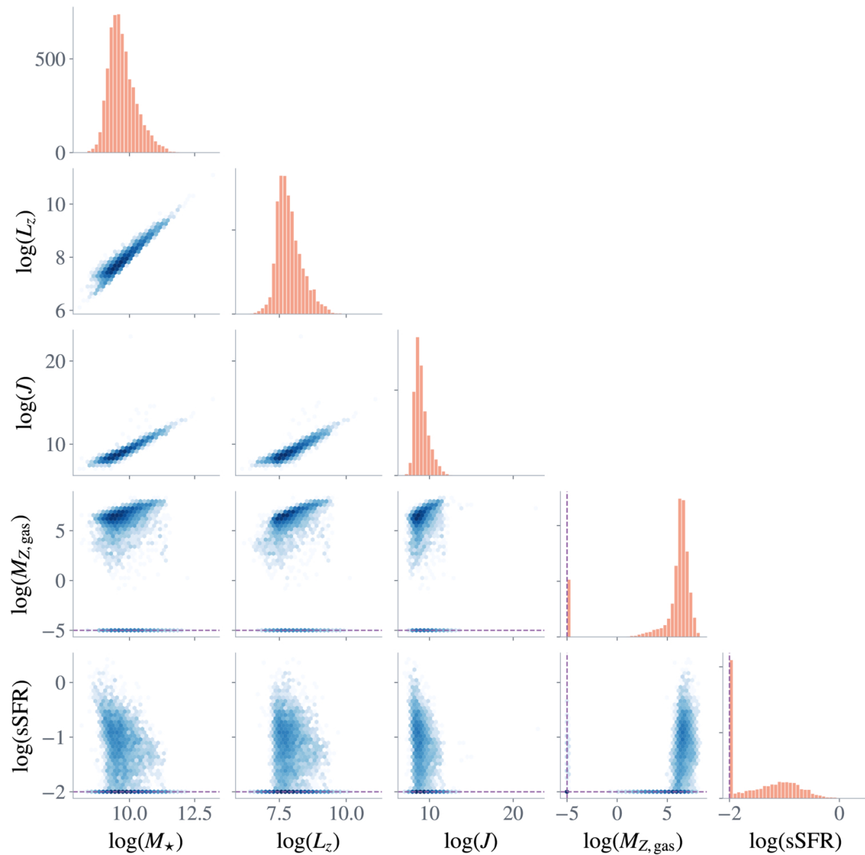
Figure 1. from Xuejie Li et al 2026 Astrophys. J. Suppl. 286 doi:10.3847/1538-4365/ae9a75 https://dx.doi.org/10.3847/1538-4365/ae9a75 © 2026. The Author(s). Published by the American Astronomical Society.
