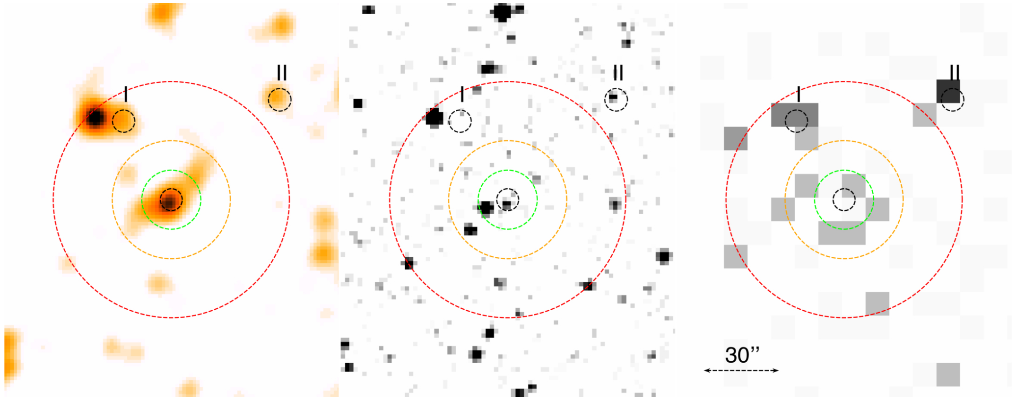
Figure 2. from Alessandro Maselli et al 2026 Astrophys. J. Suppl. 286 doi:10.3847/1538-4365/ae9955 https://dx.doi.org/10.3847/1538-4365/ae9955 © 2026. The Author(s). Published by the American Astronomical Society.
