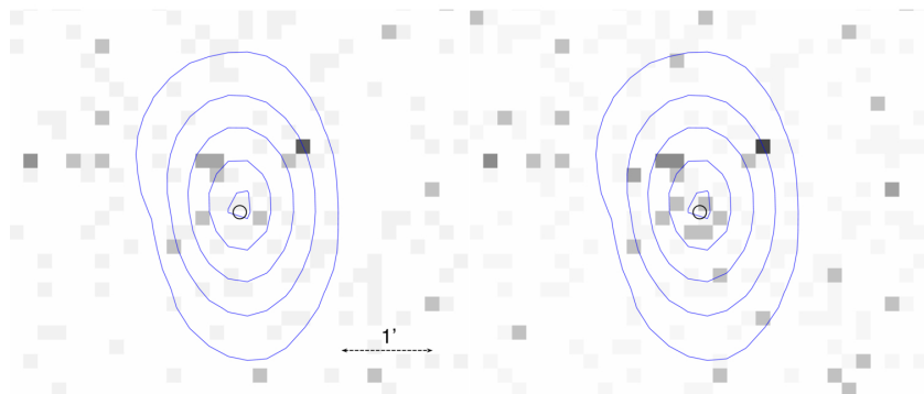
(e) MRC B2032–350 / G4Jy 1640
