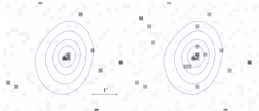
(c) MRC B1817–391 / G4Jy 1474
