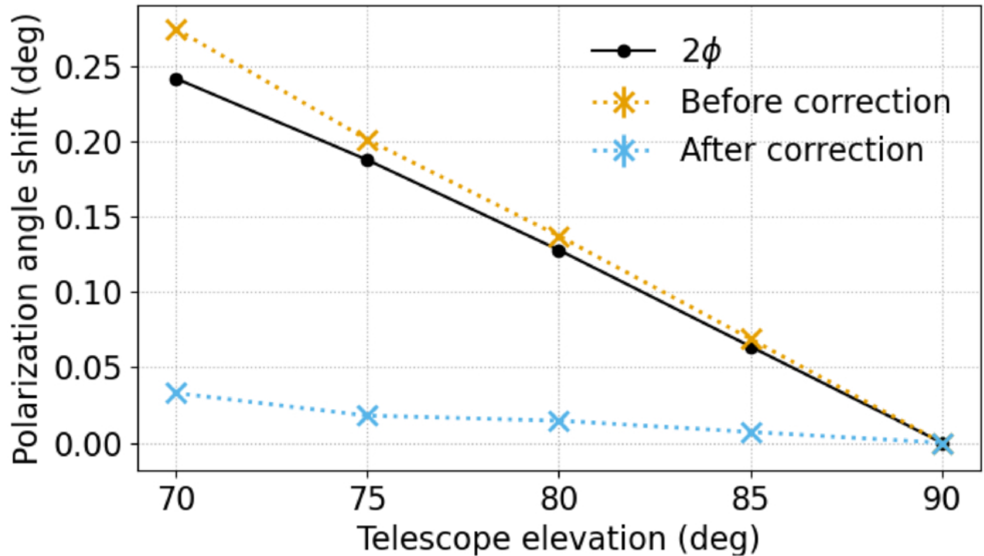
Figure 9. from Kyohei Yamada et al 2026 Astrophys. J. Suppl. 286 doi:10.3847/1538-4365/ae9934 https://dx.doi.org/10.3847/1538-4365/ae9934 © 2026. The Author(s). Published by the American Astronomical Society.
