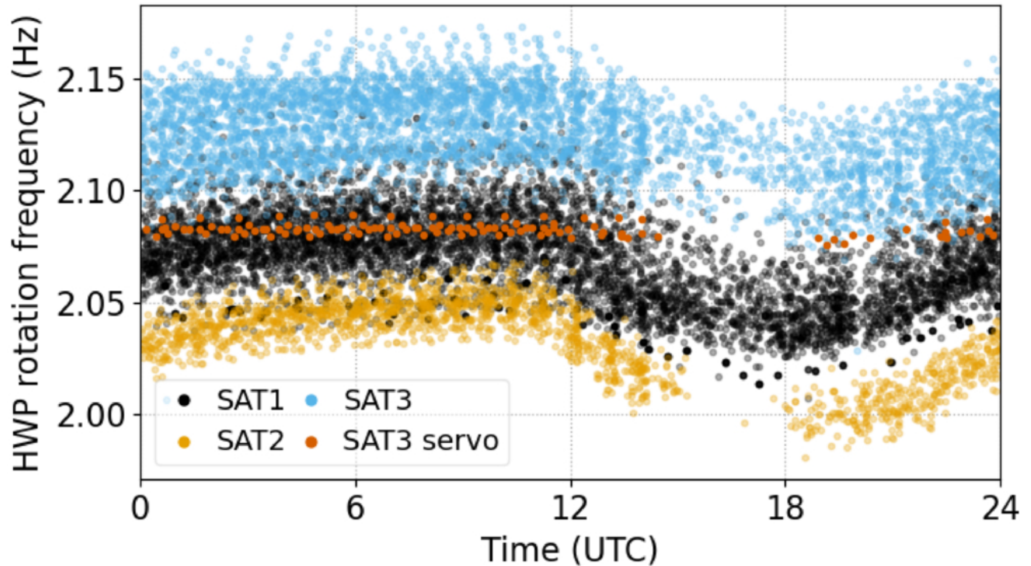
Figure 8. from Kyohei Yamada et al 2026 Astrophys. J. Suppl. 286 doi:10.3847/1538-4365/ae9934 https://dx.doi.org/10.3847/1538-4365/ae9934 © 2026. The Author(s). Published by the American Astronomical Society.
