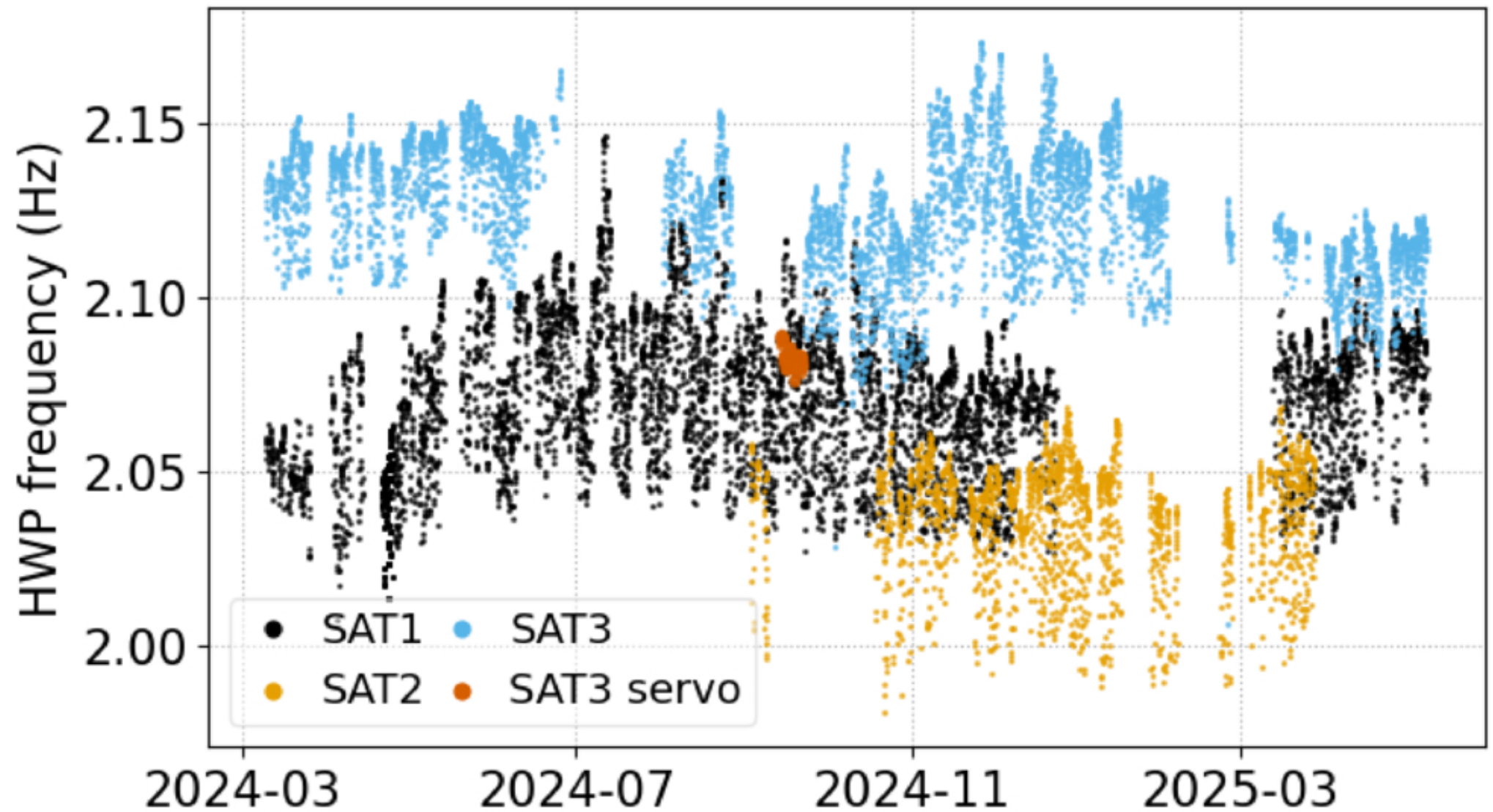
Figure 6. from Kyohei Yamada et al 2026 Astrophys. J. Suppl. 286 doi:10.3847/1538-4365/ae9934 https://dx.doi.org/10.3847/1538-4365/ae9934 © 2026. The Author(s). Published by the American Astronomical Society.
