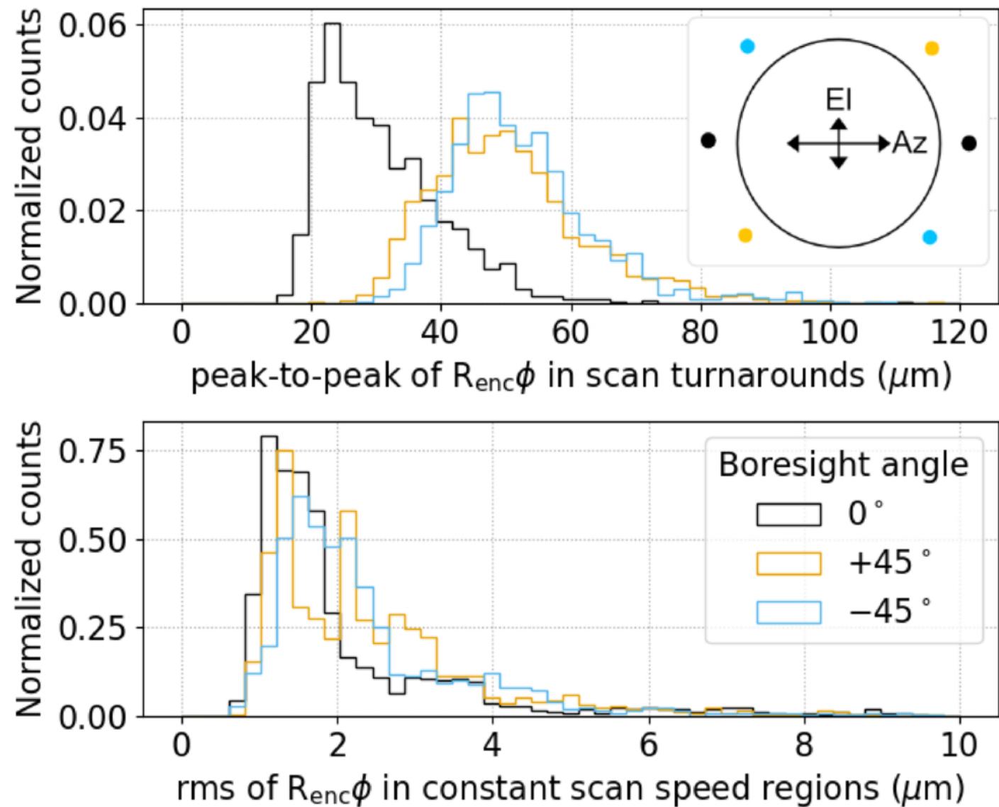
Figure 10. from Kyohei Yamada et al 2026 Astrophys. J. Suppl. 286 doi:10.3847/1538-4365/ae9934 https://dx.doi.org/10.3847/1538-4365/ae9934 © 2026. The Author(s). Published by the American Astronomical Society.
