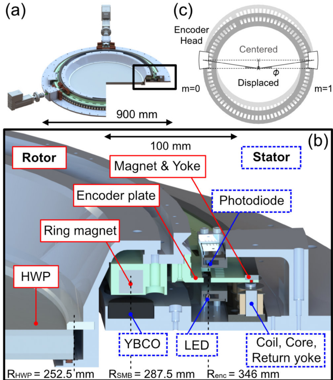
Figure 1. from Kyohei Yamada et al 2026 Astrophys. J. Suppl. 286 doi:10.3847/1538-4365/ae9934 https://dx.doi.org/10.3847/1538-4365/ae9934 © 2026. The Author(s). Published by the American Astronomical Society.
