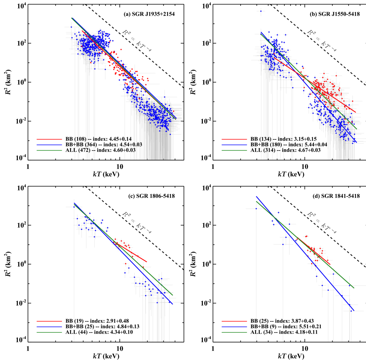
Figure 9. from Matt Godwin et al 2026 Astrophys. J. Suppl. 286 doi:10.3847/1538-4365/ae9904 https://dx.doi.org/10.3847/1538-4365/ae9904 © 2026. The Author(s). Published by the American Astronomical Society.
