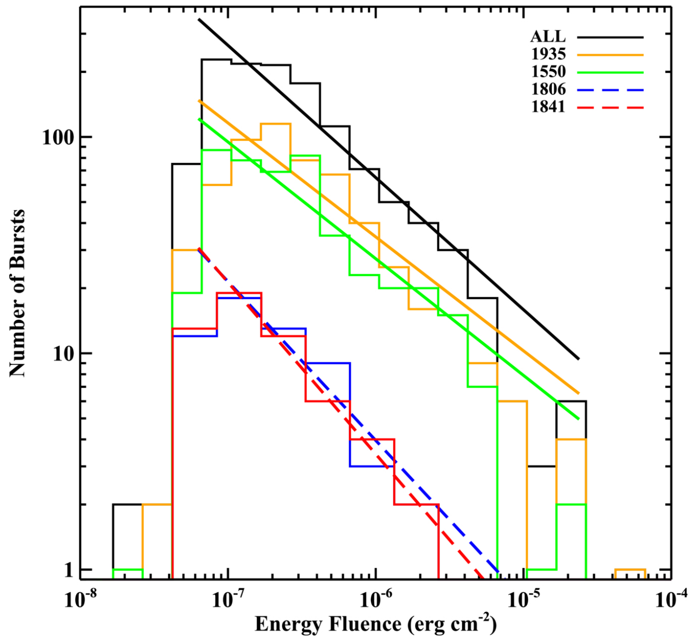
Figure 7. from Matt Godwin et al 2026 Astrophys. J. Suppl. 286 doi:10.3847/1538-4365/ae9904 https://dx.doi.org/10.3847/1538-4365/ae9904 © 2026. The Author(s). Published by the American Astronomical Society.
