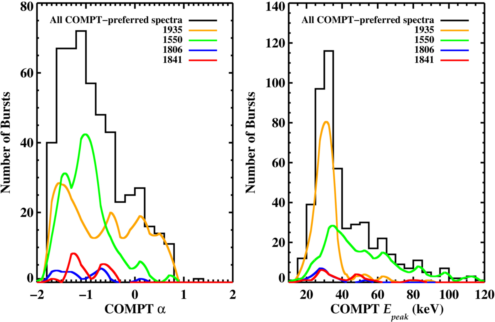
Figure 5. from Matt Godwin et al 2026 Astrophys. J. Suppl. 286 doi:10.3847/1538-4365/ae9904 https://dx.doi.org/10.3847/1538-4365/ae9904 © 2026. The Author(s). Published by the American Astronomical Society.
