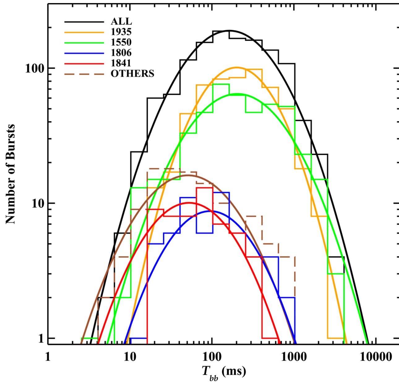
Figure 2. from Matt Godwin et al 2026 Astrophys. J. Suppl. 286 doi:10.3847/1538-4365/ae9904 https://dx.doi.org/10.3847/1538-4365/ae9904 © 2026. The Author(s). Published by the American Astronomical Society.
