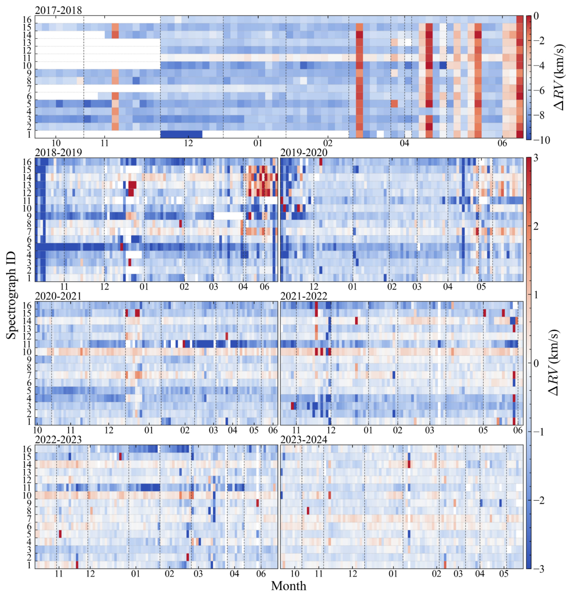
Figure A1. from Jinming Zhang and Haibo Yuan 2026 Astrophys. J. Suppl. 286 doi:10.3847/1538-4365/ae985e https://dx.doi.org/10.3847/1538-4365/ae985e © 2026. The Author(s). Published by the American Astronomical Society.
