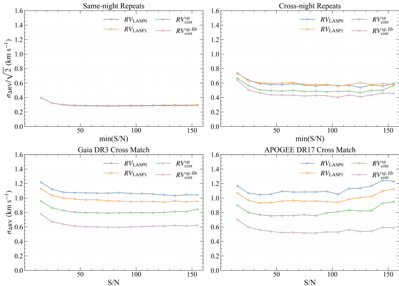
Figure 5. from Jinming Zhang and Haibo Yuan 2026 Astrophys. J. Suppl. 286 doi:10.3847/1538-4365/ae985e https://dx.doi.org/10.3847/1538-4365/ae985e © 2026. The Author(s). Published by the American Astronomical Society.
