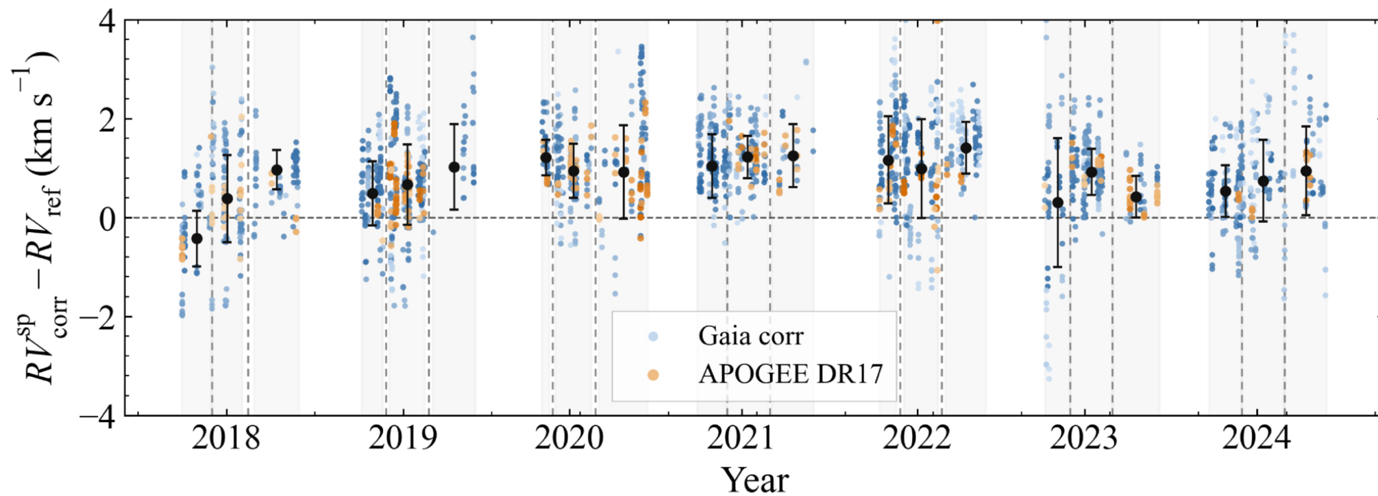
Figure 3. from Jinming Zhang and Haibo Yuan 2026 Astrophys. J. Suppl. 286 doi:10.3847/1538-4365/ae985e https://dx.doi.org/10.3847/1538-4365/ae985e © 2026. The Author(s). Published by the American Astronomical Society.
