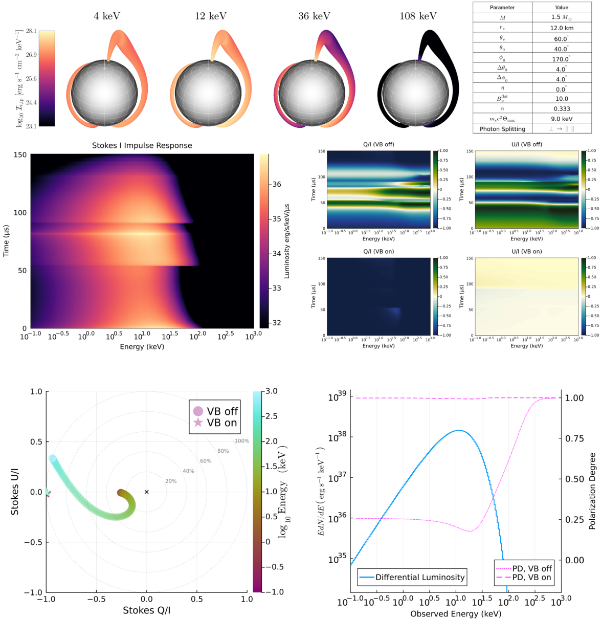
Figure 9. from Zorawar Wadiasingh et al 2026 Astrophys. J. Suppl. 286 doi:10.3847/1538-4365/ae9754 https://dx.doi.org/10.3847/1538-4365/ae9754 © 2026. The Author(s). Published by the American Astronomical Society.
