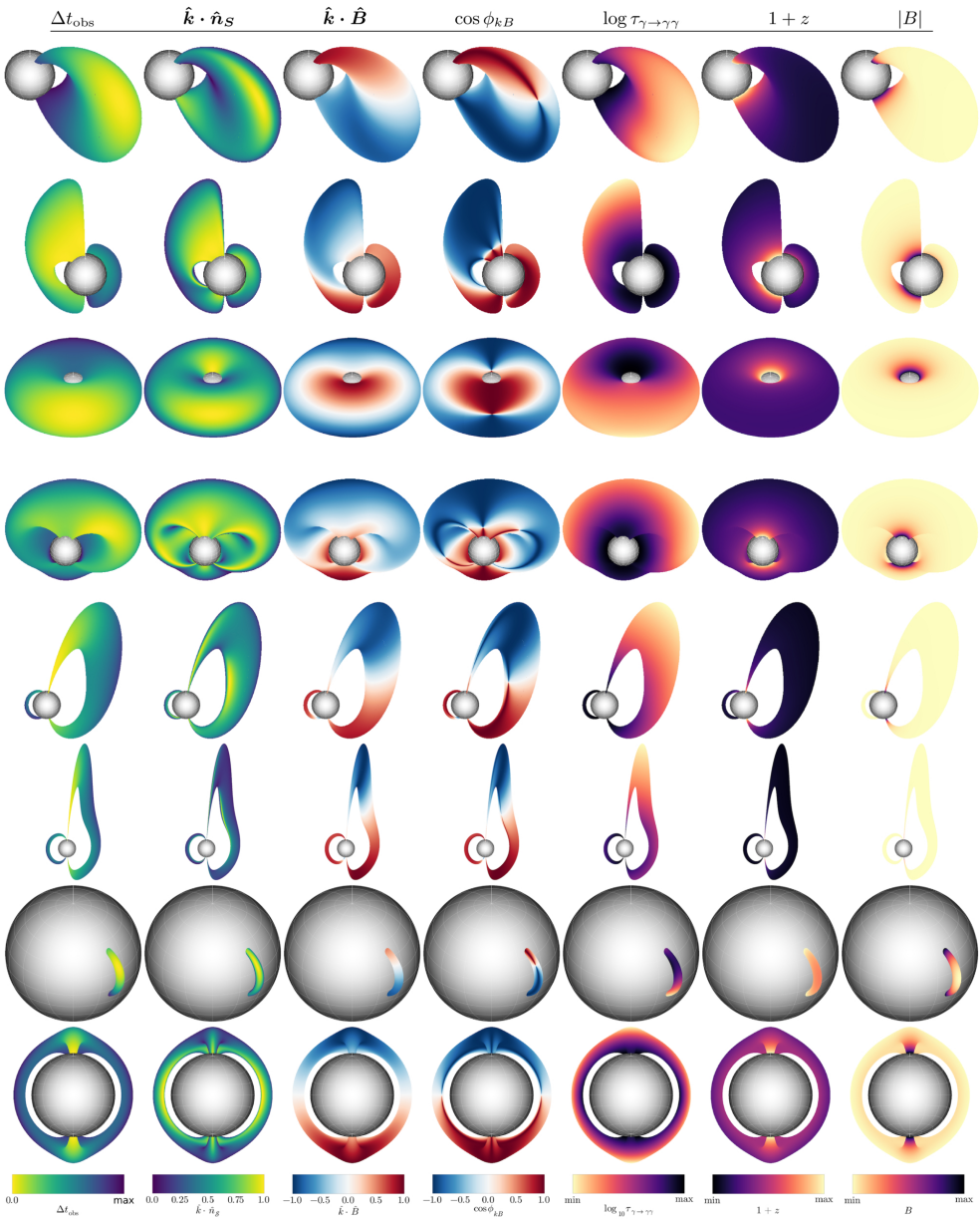
Figure 2. from Zorawar Wadiasingh et al 2026 Astrophys. J. Suppl. 286 doi:10.3847/1538-4365/ae9754 https://dx.doi.org/10.3847/1538-4365/ae9754 © 2026. The Author(s). Published by the American Astronomical Society.
