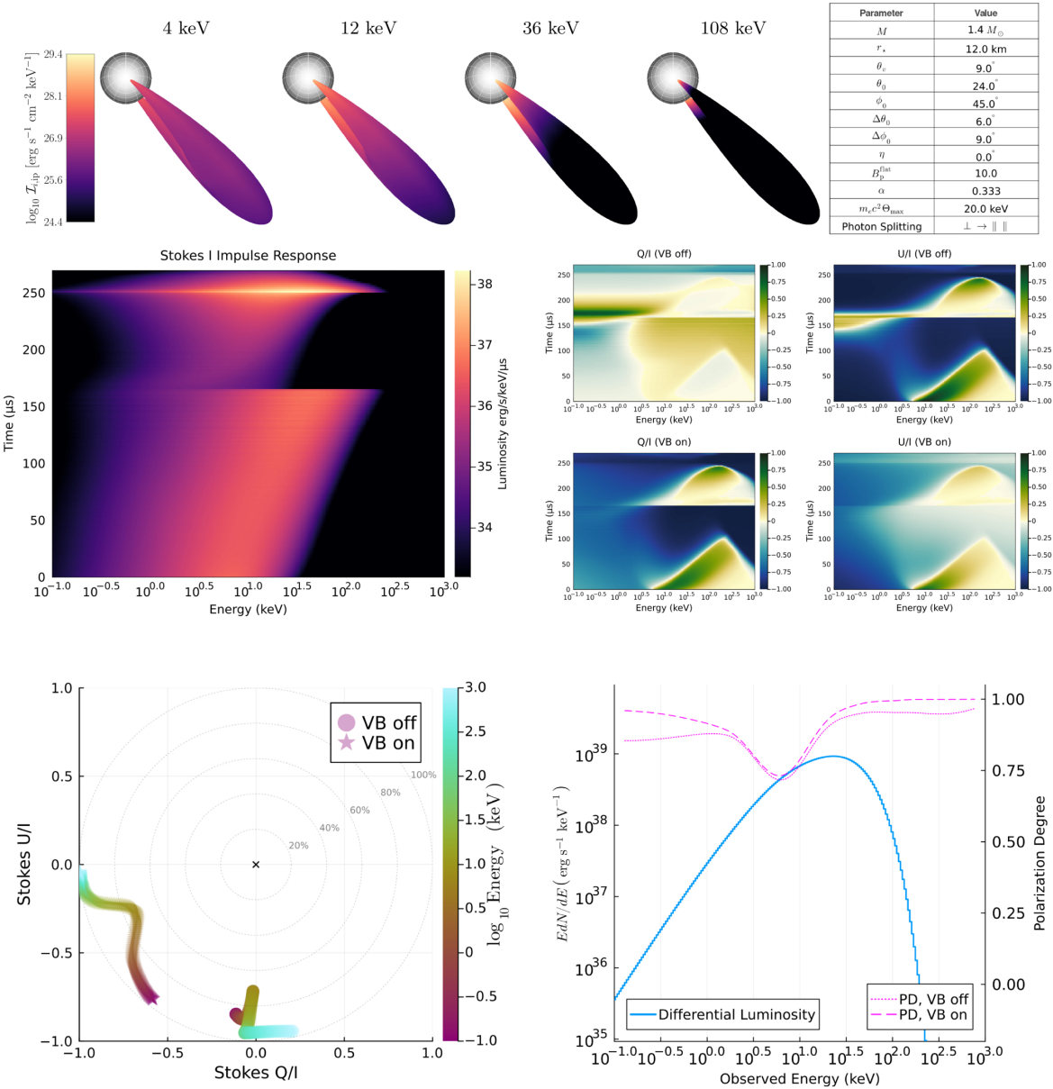
Figure 16. from Zorawar Wadiasingh et al 2026 Astrophys. J. Suppl. 286 doi:10.3847/1538-4365/ae9754 https://dx.doi.org/10.3847/1538-4365/ae9754 © 2026. The Author(s). Published by the American Astronomical Society.
