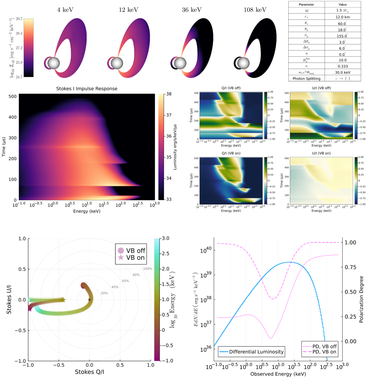
Figure 14. from Zorawar Wadiasingh et al 2026 Astrophys. J. Suppl. 286 doi:10.3847/1538-4365/ae9754 https://dx.doi.org/10.3847/1538-4365/ae9754 © 2026. The Author(s). Published by the American Astronomical Society.
