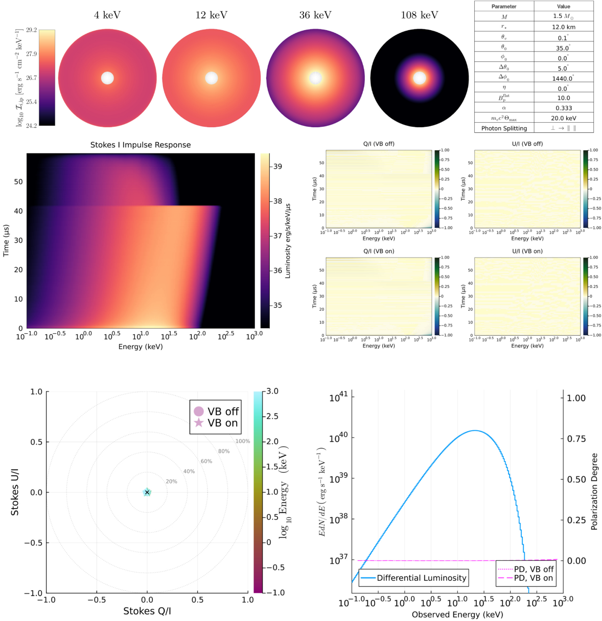
Figure 11. from Zorawar Wadiasingh et al 2026 Astrophys. J. Suppl. 286 doi:10.3847/1538-4365/ae9754 https://dx.doi.org/10.3847/1538-4365/ae9754 © 2026. The Author(s). Published by the American Astronomical Society.
