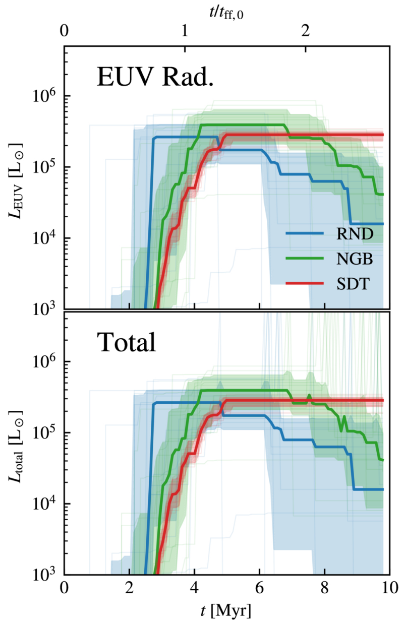
Figure 8. from Yunwei Deng et al 2026 Astrophys. J. Suppl. 286 doi:10.3847/1538-4365/ae974d https://dx.doi.org/10.3847/1538-4365/ae974d © 2026. The Author(s). Published by the American Astronomical Society.
