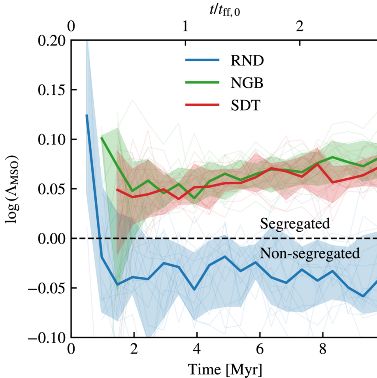
Figure 7. from Yunwei Deng et al 2026 Astrophys. J. Suppl. 286 doi:10.3847/1538-4365/ae974d https://dx.doi.org/10.3847/1538-4365/ae974d © 2026. The Author(s). Published by the American Astronomical Society.
