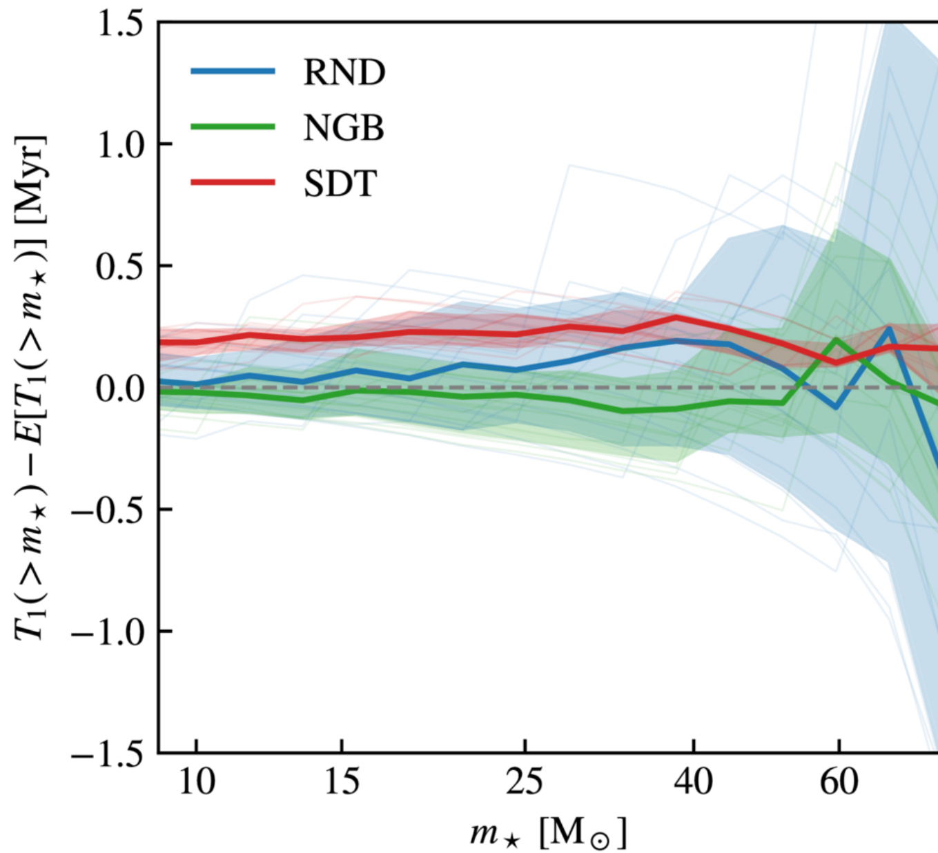
Figure 6. from Yunwei Deng et al 2026 Astrophys. J. Suppl. 286 doi:10.3847/1538-4365/ae974d https://dx.doi.org/10.3847/1538-4365/ae974d © 2026. The Author(s). Published by the American Astronomical Society.
