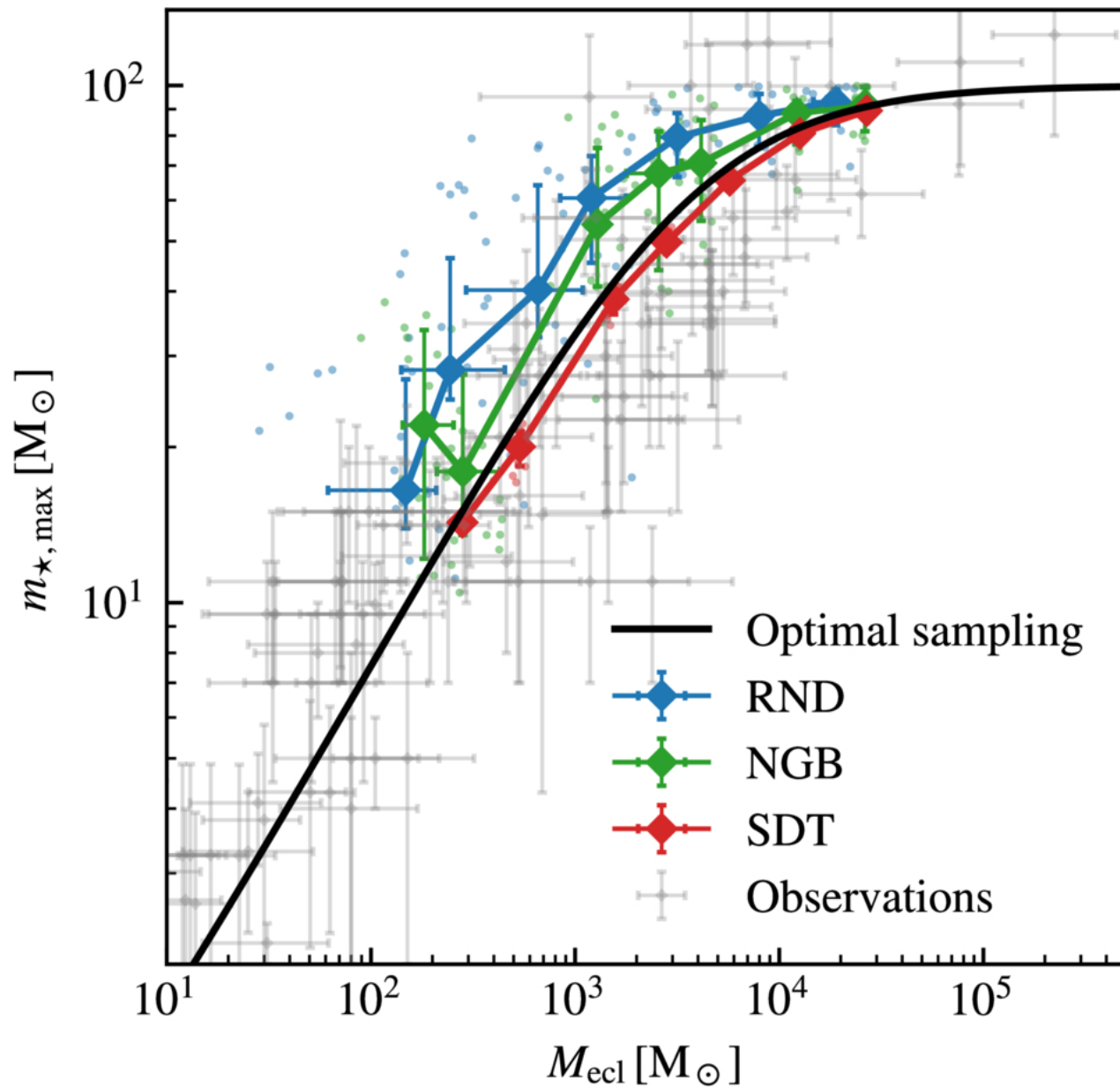
Figure 4. from Yunwei Deng et al 2026 Astrophys. J. Suppl. 286 doi:10.3847/1538-4365/ae974d https://dx.doi.org/10.3847/1538-4365/ae974d © 2026. The Author(s). Published by the American Astronomical Society.
