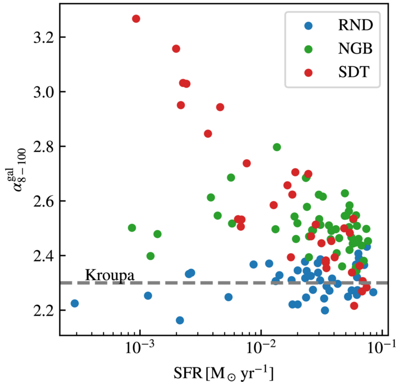
Figure 14. from Yunwei Deng et al 2026 Astrophys. J. Suppl. 286 doi:10.3847/1538-4365/ae974d https://dx.doi.org/10.3847/1538-4365/ae974d © 2026. The Author(s). Published by the American Astronomical Society.
