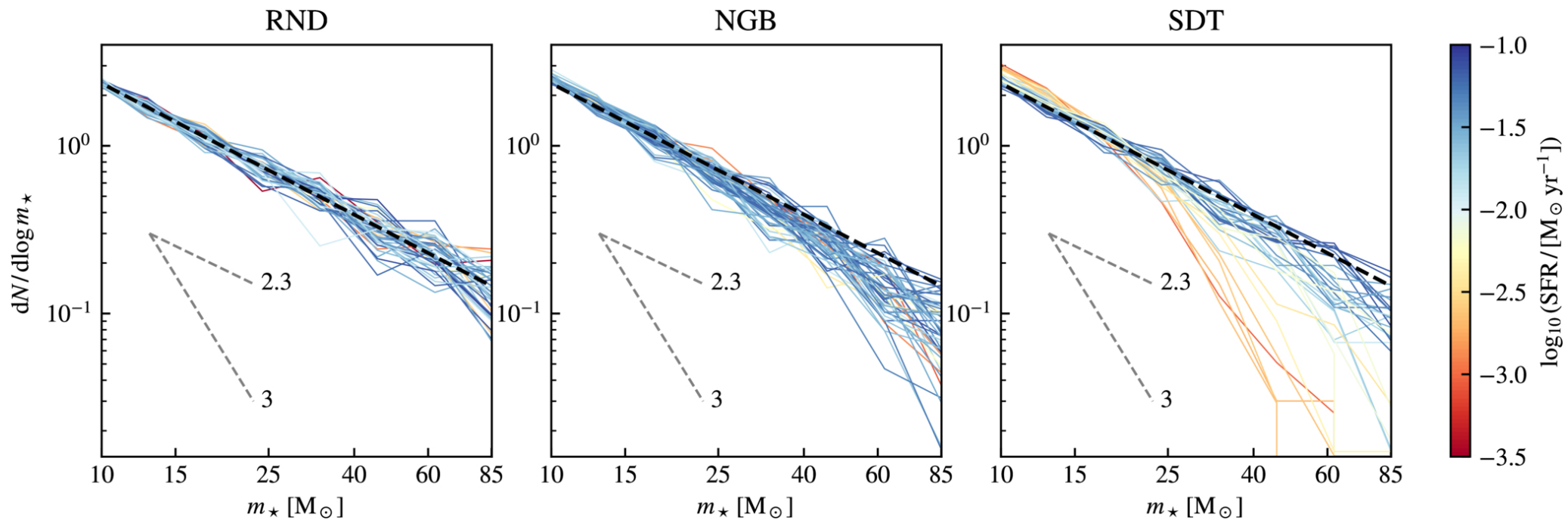
Figure 13. from Yunwei Deng et al 2026 Astrophys. J. Suppl. 286 doi:10.3847/1538-4365/ae974d https://dx.doi.org/10.3847/1538-4365/ae974d © 2026. The Author(s). Published by the American Astronomical Society.
