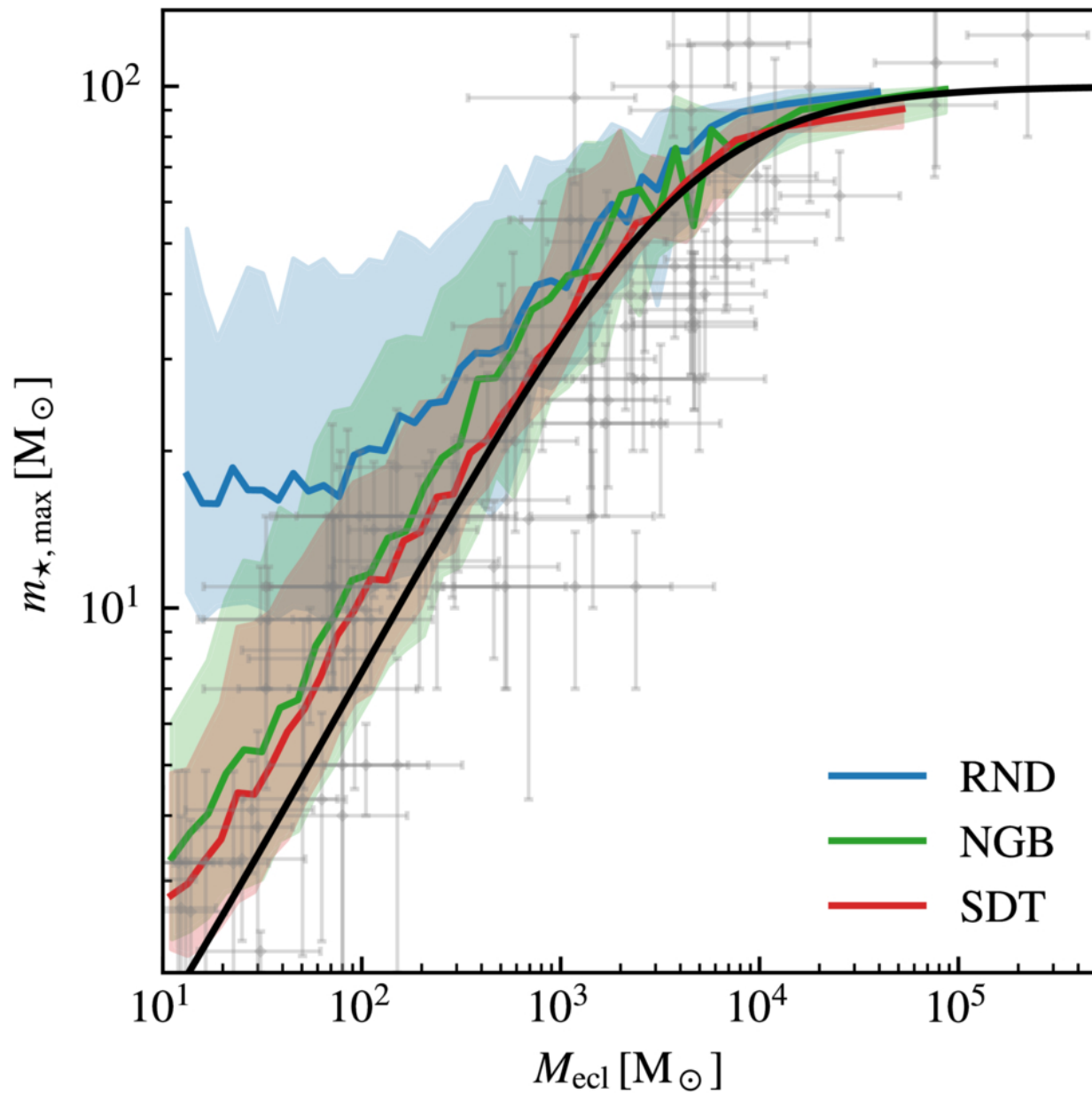
Figure 12. from Yunwei Deng et al 2026 Astrophys. J. Suppl. 286 doi:10.3847/1538-4365/ae974d https://dx.doi.org/10.3847/1538-4365/ae974d © 2026. The Author(s). Published by the American Astronomical Society.
