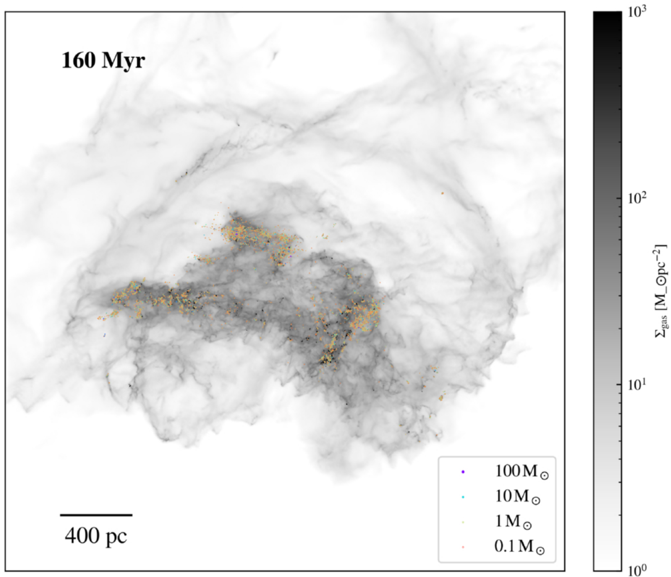
Figure 10. from Yunwei Deng et al 2026 Astrophys. J. Suppl. 286 doi:10.3847/1538-4365/ae974d https://dx.doi.org/10.3847/1538-4365/ae974d © 2026. The Author(s). Published by the American Astronomical Society.
