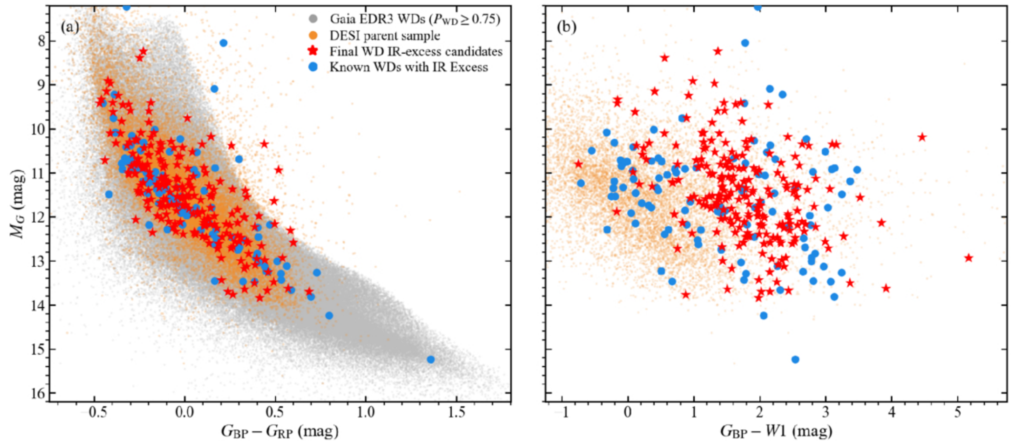
Figure 7. from Nanlu Huang et al 2026 Astrophys. J. Suppl. 286 doi:10.3847/1538-4365/ae9550 https://dx.doi.org/10.3847/1538-4365/ae9550 © 2026. The Author(s). Published by the American Astronomical Society.
