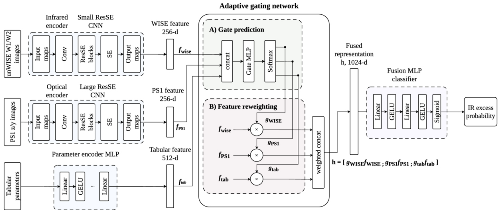
Figure 3. from Nanlu Huang et al 2026 Astrophys. J. Suppl. 286 doi:10.3847/1538-4365/ae9550 https://dx.doi.org/10.3847/1538-4365/ae9550 © 2026. The Author(s). Published by the American Astronomical Society.
