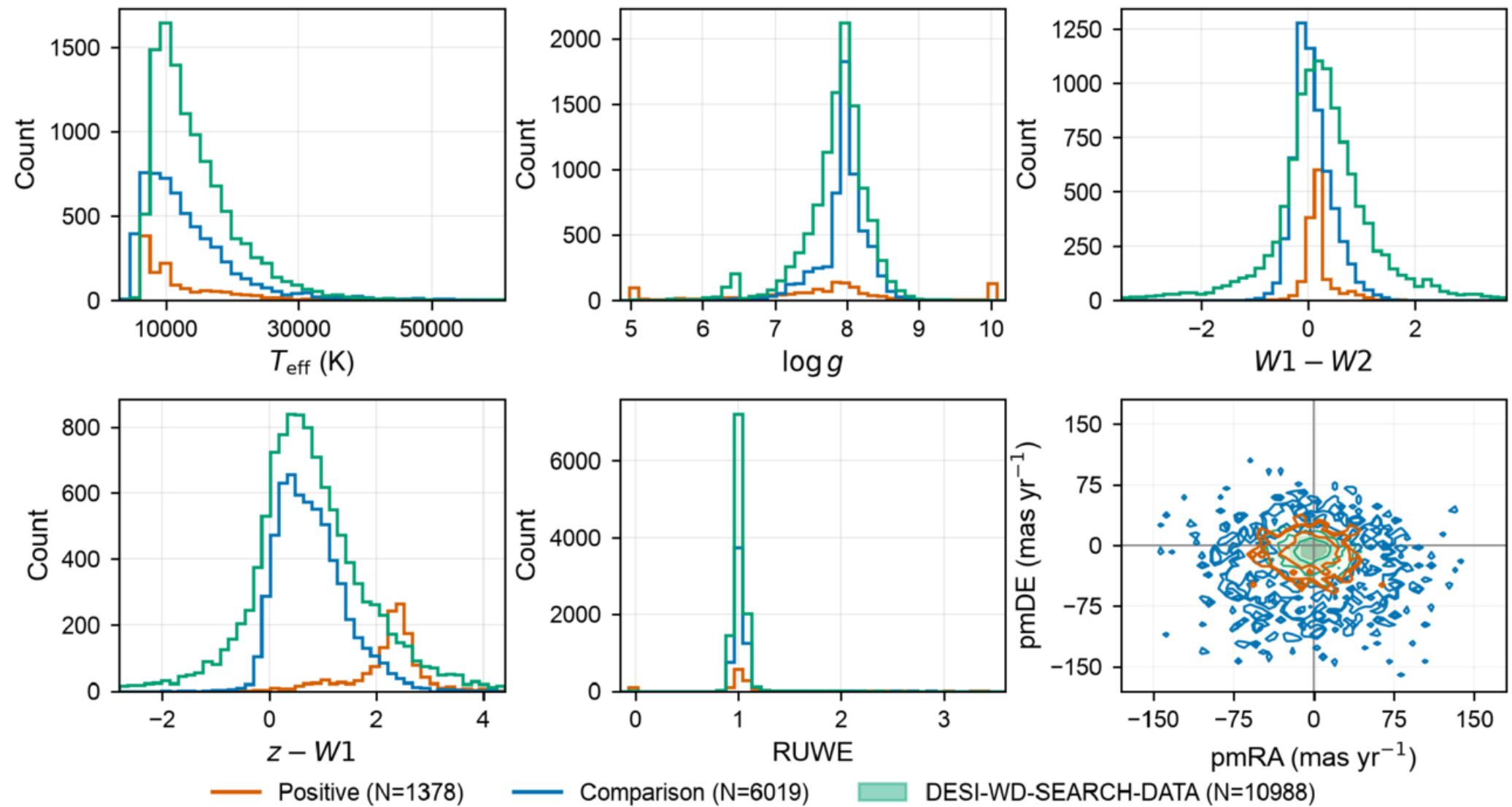
Figure 2. from Nanlu Huang et al 2026 Astrophys. J. Suppl. 286 doi:10.3847/1538-4365/ae9550 https://dx.doi.org/10.3847/1538-4365/ae9550 © 2026. The Author(s). Published by the American Astronomical Society.
