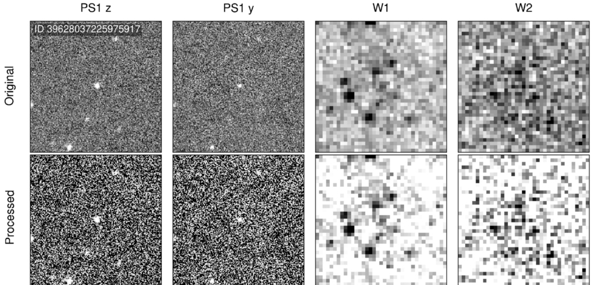
Figure 1. from Nanlu Huang et al 2026 Astrophys. J. Suppl. 286 doi:10.3847/1538-4365/ae9550 https://dx.doi.org/10.3847/1538-4365/ae9550 © 2026. The Author(s). Published by the American Astronomical Society.
