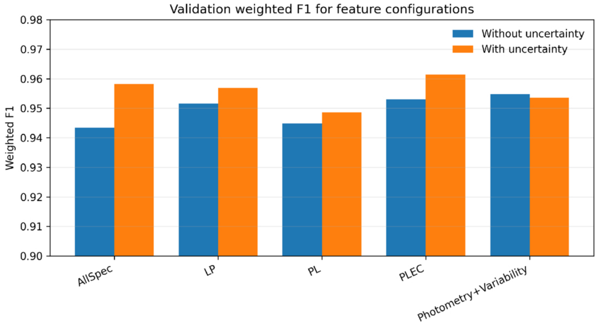
Figure 7. from Jingtian Zhu et al 2026 Astrophys. J. Suppl. 286 doi:10.3847/1538-4365/ae91e8 https://dx.doi.org/10.3847/1538-4365/ae91e8 © 2026. The Author(s). Published by the American Astronomical Society.
